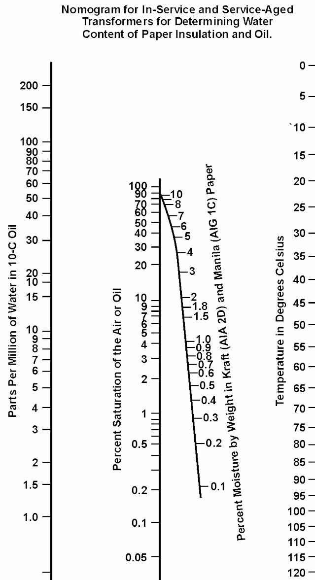
Figure 55 – Water Content of Paper and Oil Nomogram.
