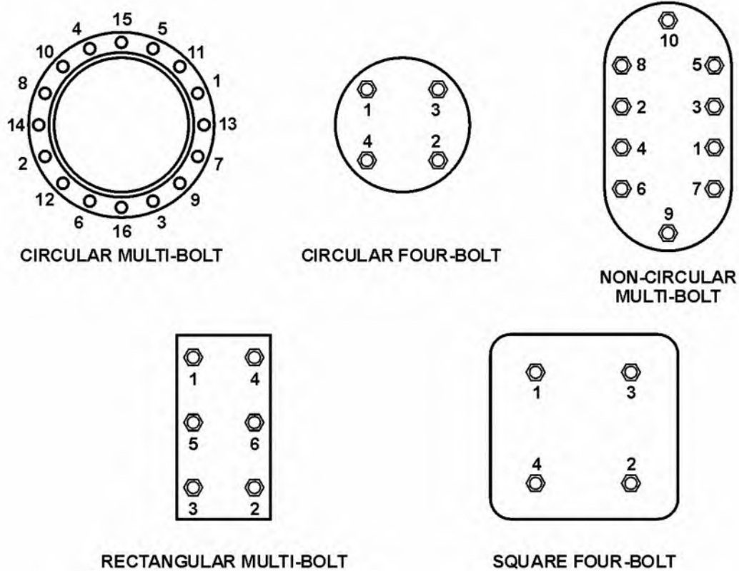
Figure 47 – Bolt Tightening Sequences.
